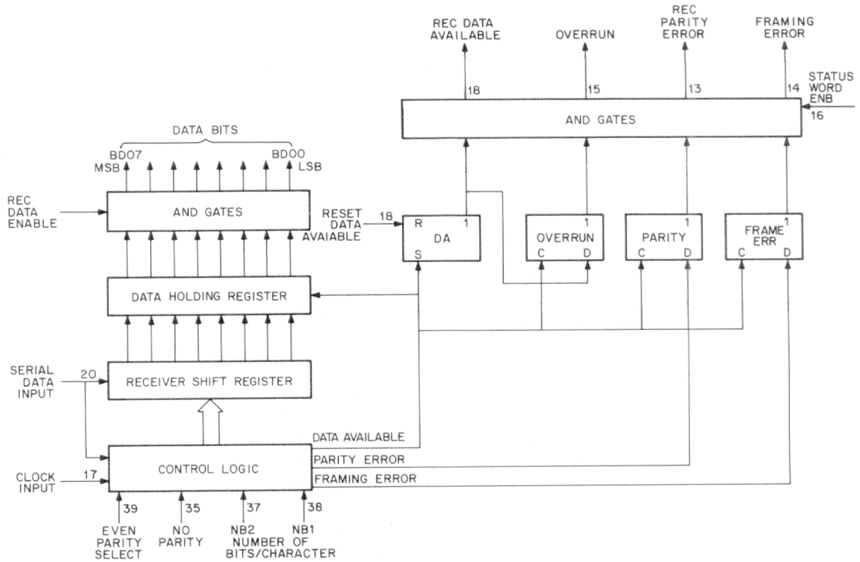
Figure C-3 UART Receiver, Block Diagram and Simplified Timing Diagram
