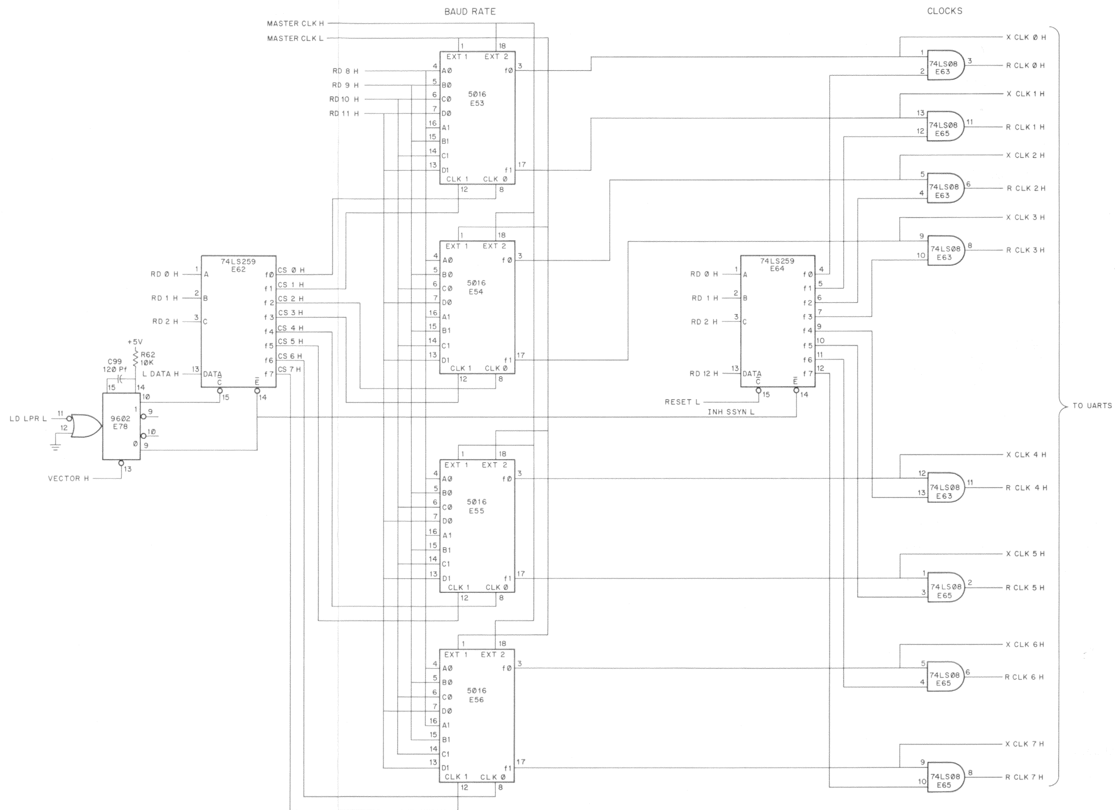
Figure 4-18 LPR Diagram
