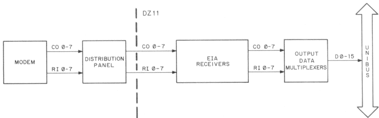
Figure 4-20 MSR Diagram
