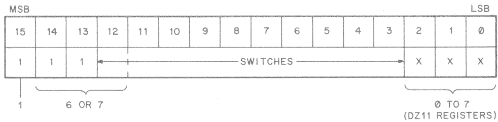
Figure 4-5 Address Word Format
