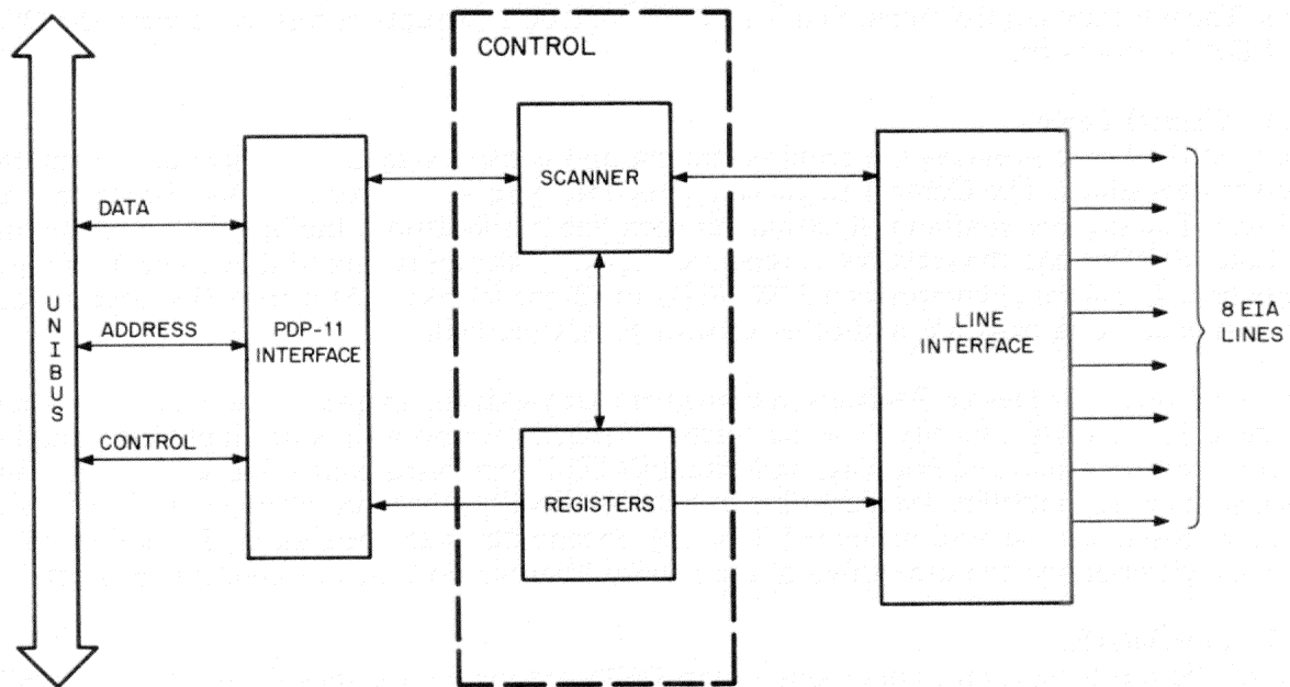
Figure 1-7 General Functional Block Diagram
