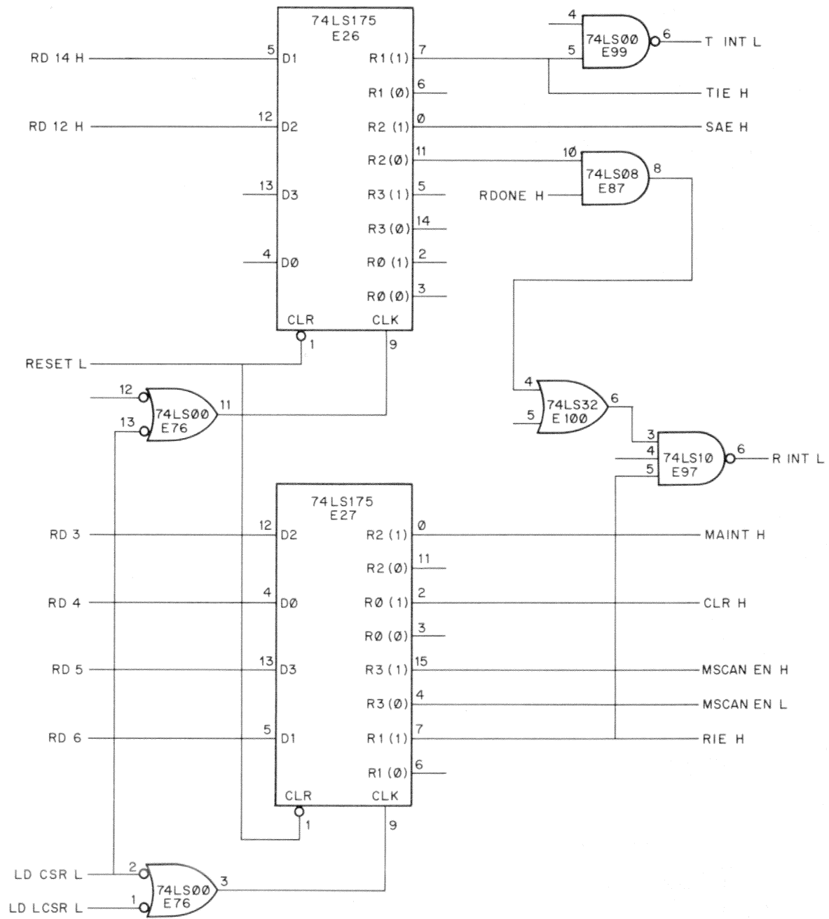
Figure 4-17 CSR Diagram
