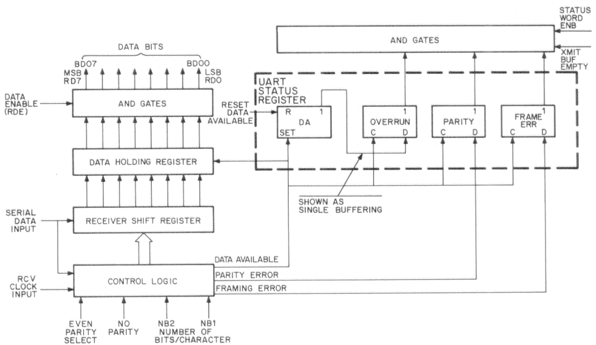
Figure 4-21 UART RCVR Block Diagram
