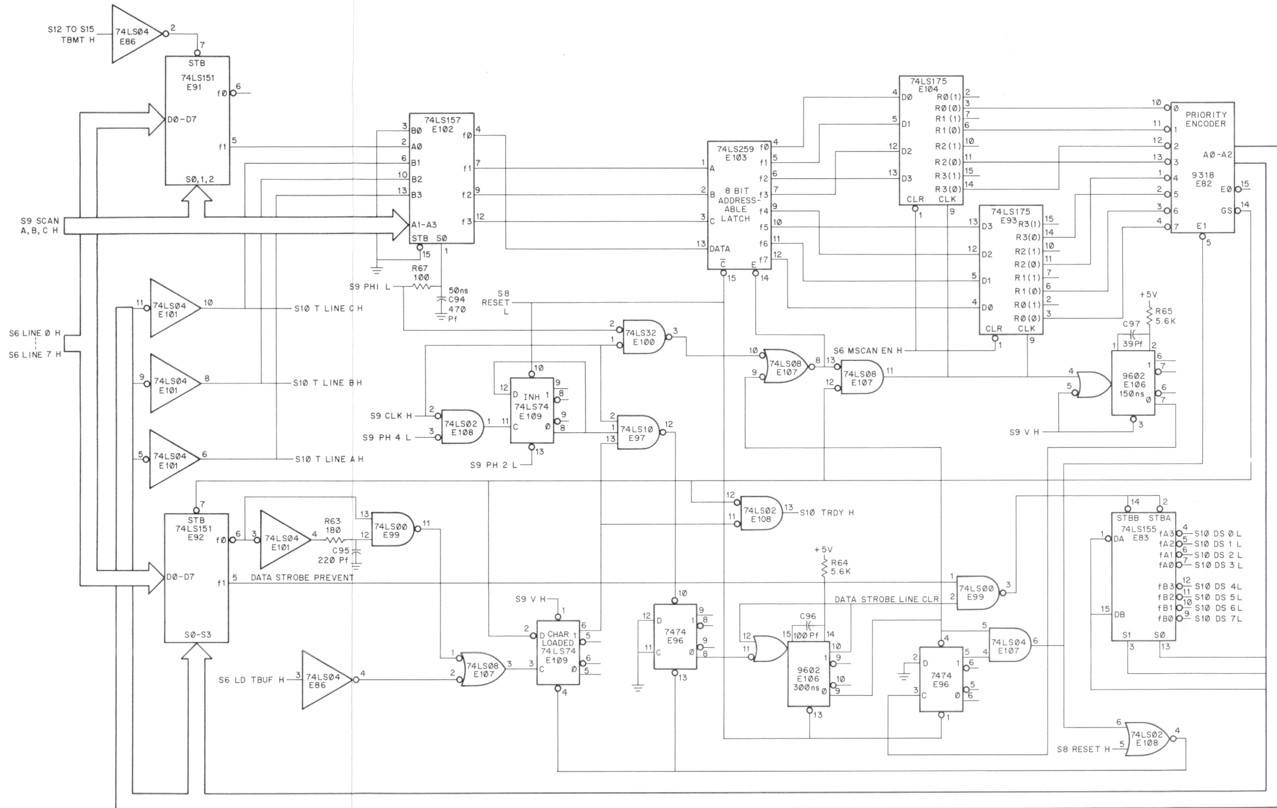
Figure 4-14 Transmit Control Logic
