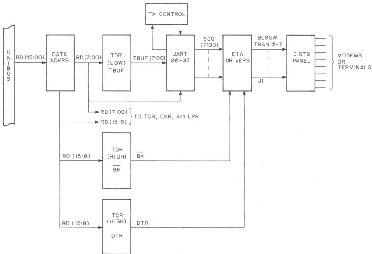
Figure 4-2 Unibus-to-Modem Data Flow (Transmit)
