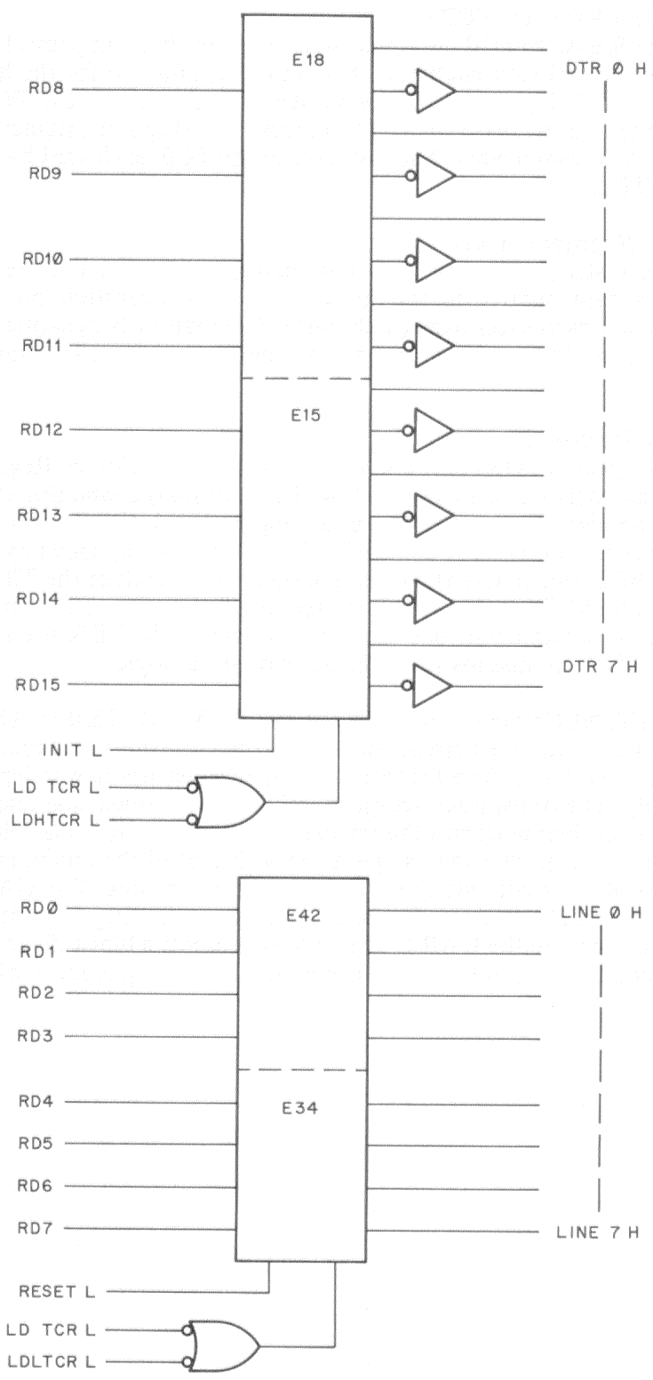
Figure 4-19 TCR Diagram
