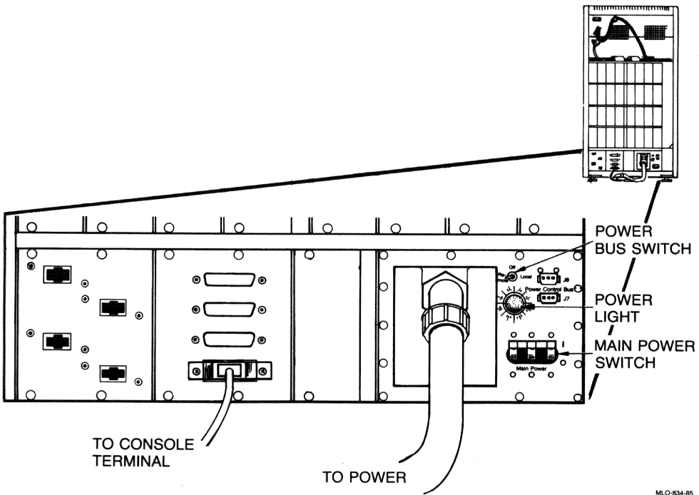
Figure 1-7: Back View of 12-Slot Main Cabinet with Panel Removed
