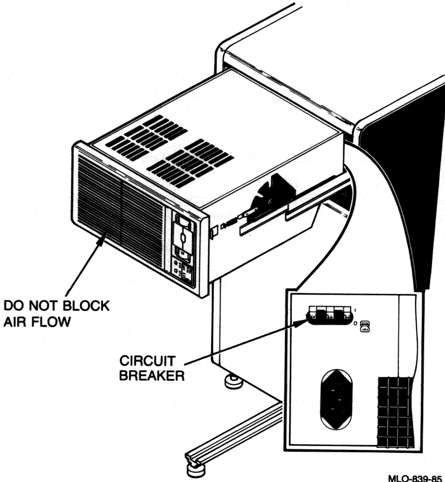
Figure 1-11: Circuit Breaker Switch for 12-Slot System
