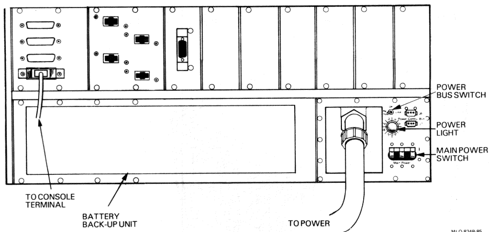
Figure 1-8: Back View of 24-Slot Main Cabinet with Panel Removed
