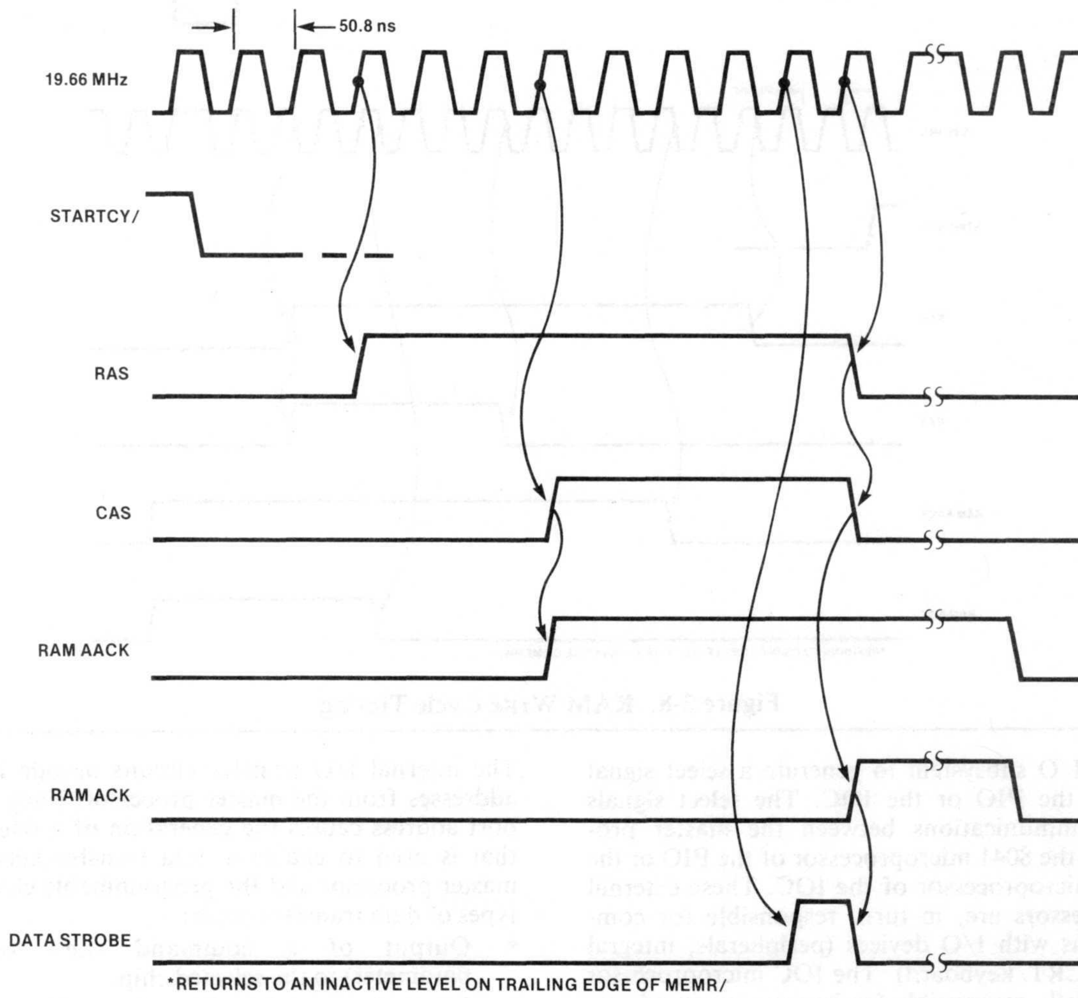
Figure 2-7. RAM Read Cycle Timing
