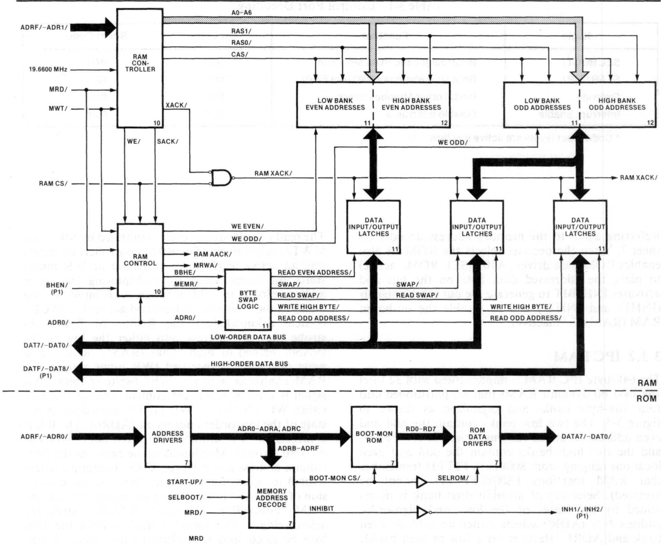
Figure 3-5. IPC Memory Subsystem Block Diagram
