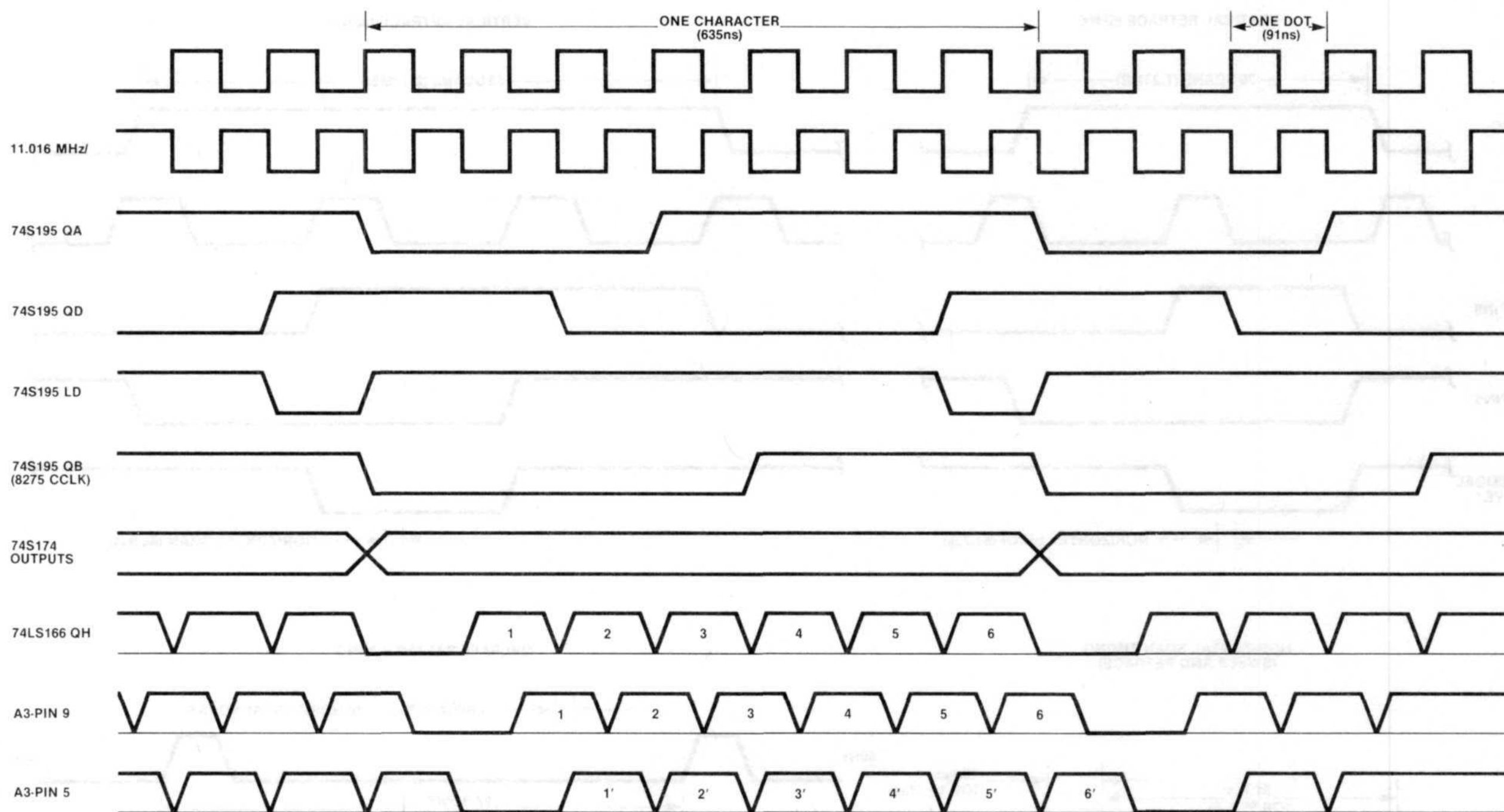
Figure 4-7. Dot Pattern Timing
