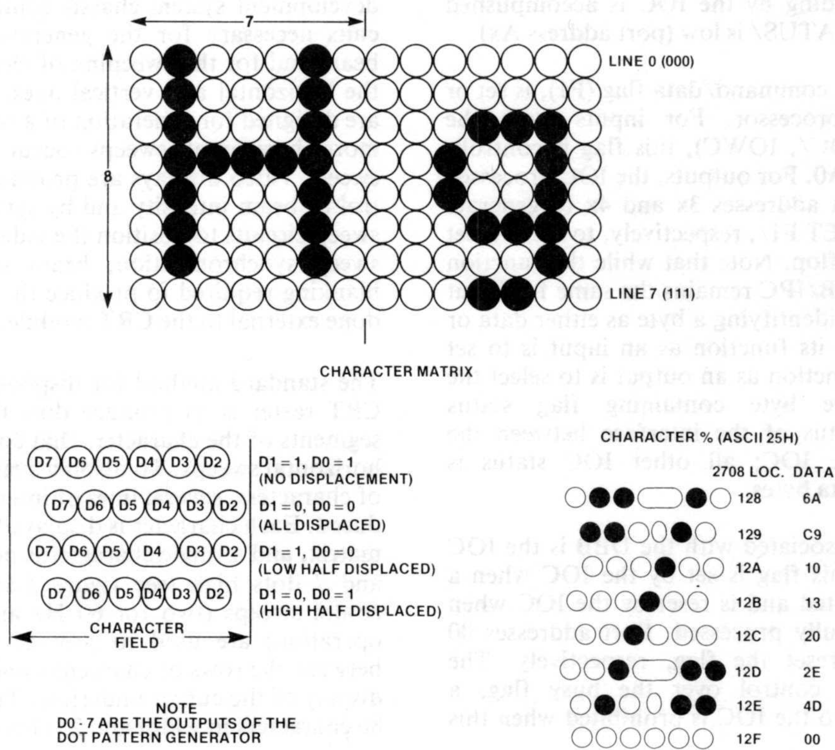
Figure 4-6. Character Display Matrix
