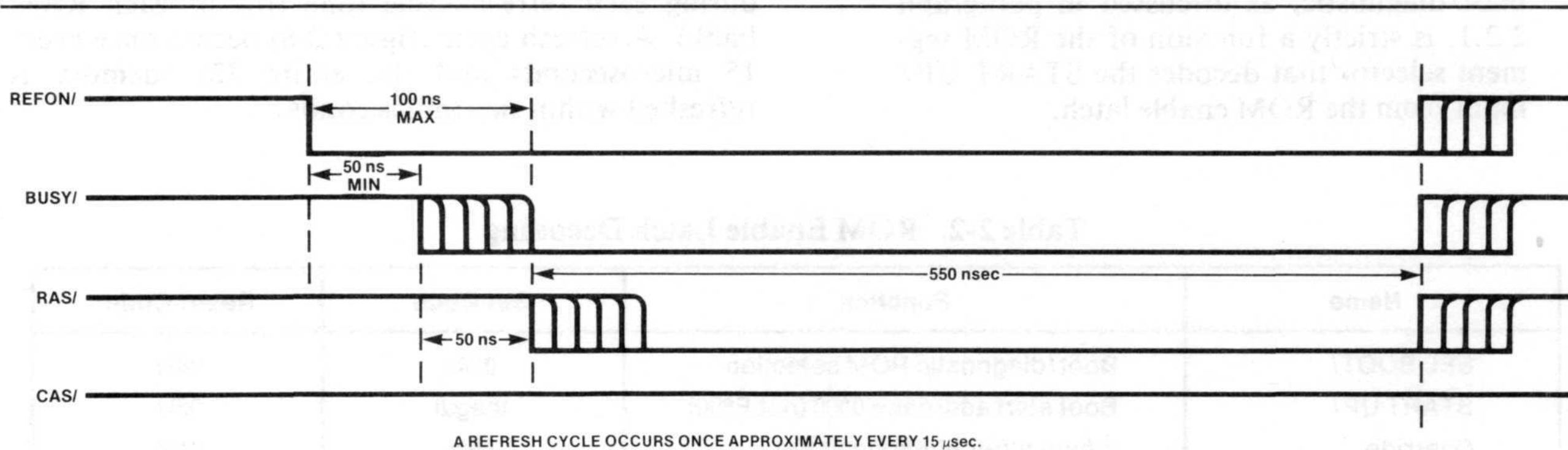
Figure 2-6. RAM Refresh Cycle Timing
