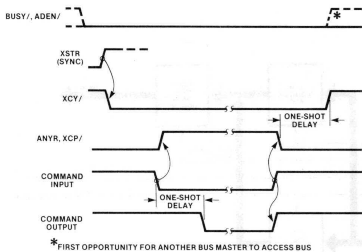
Figure 2-4. Bus Control Cycle Timing 556-7
