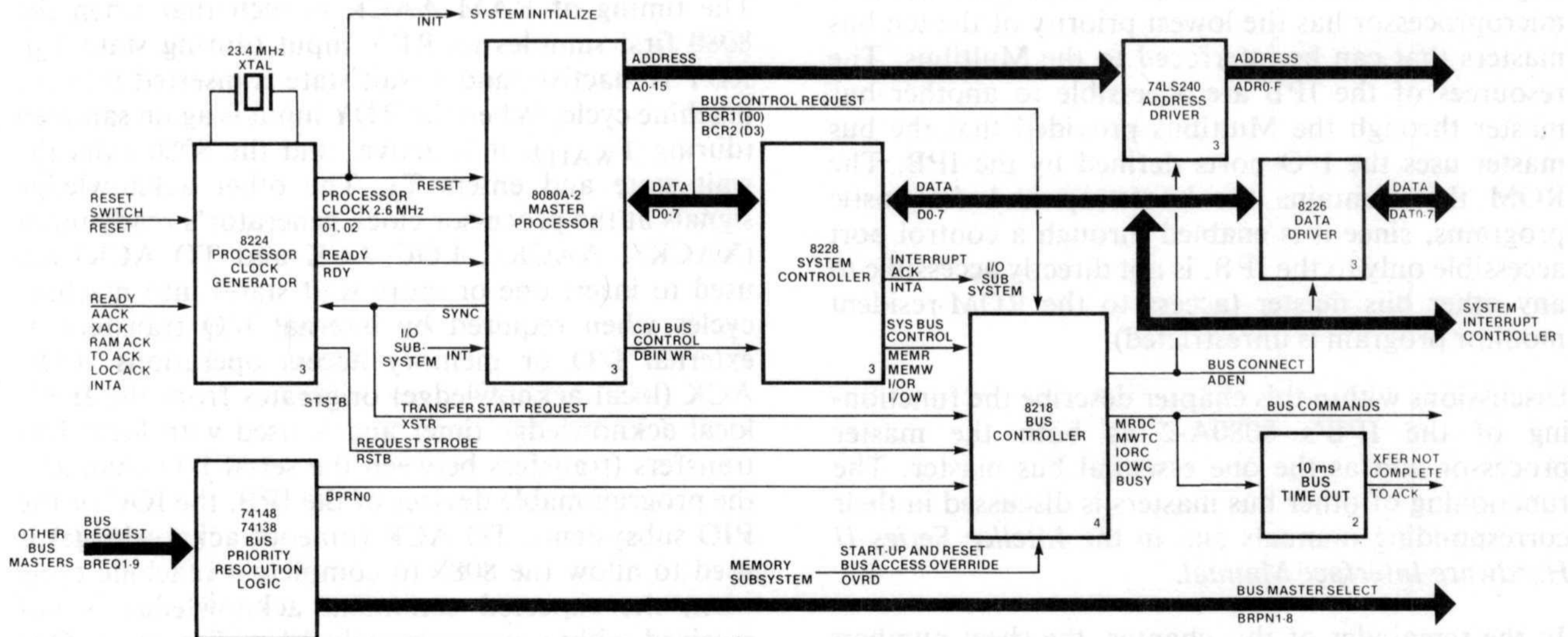
Figure 2-1. IPB Simplified Block Diagram
