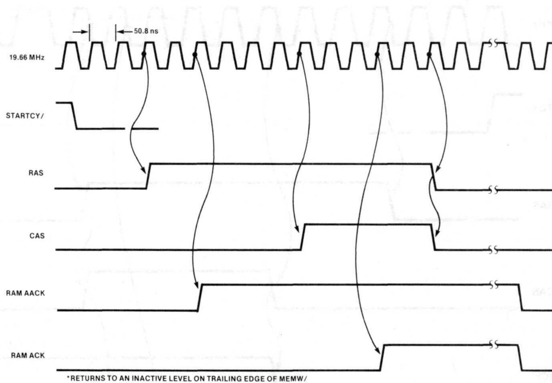
Figure 2-8. RAM Write Cycle Timing
