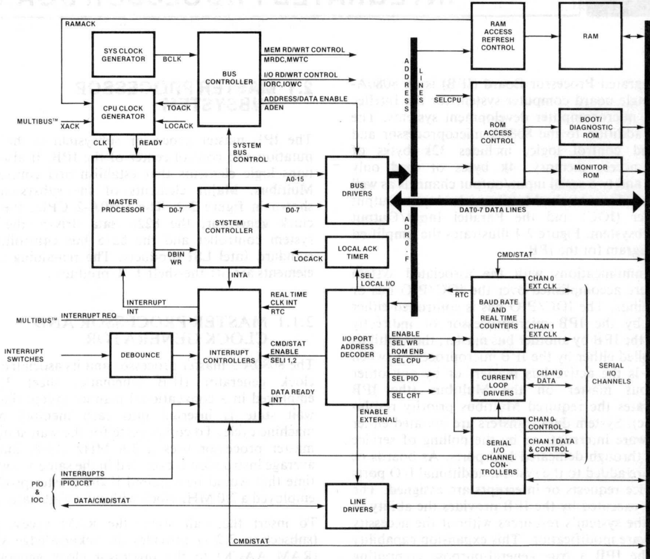
Figure 2-1. IPB Simplified Block Diagram
