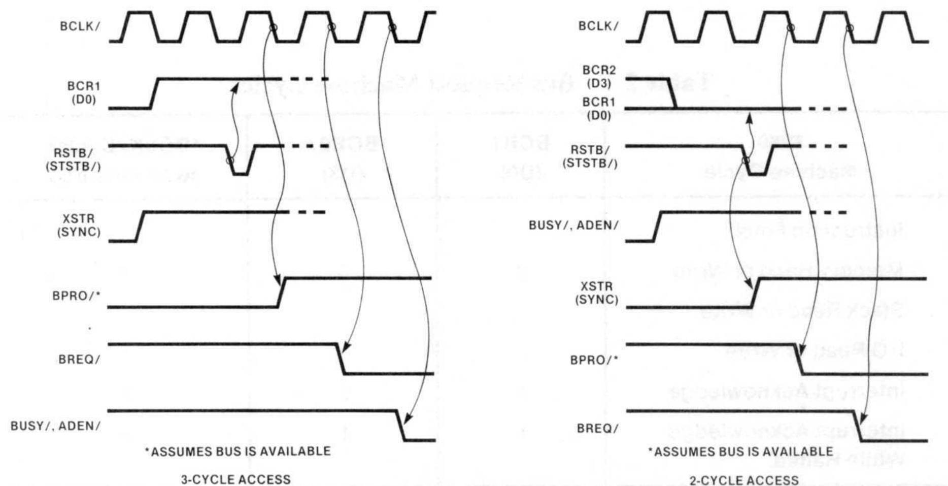
Figure 2-3. Bus Acquisition Timing
