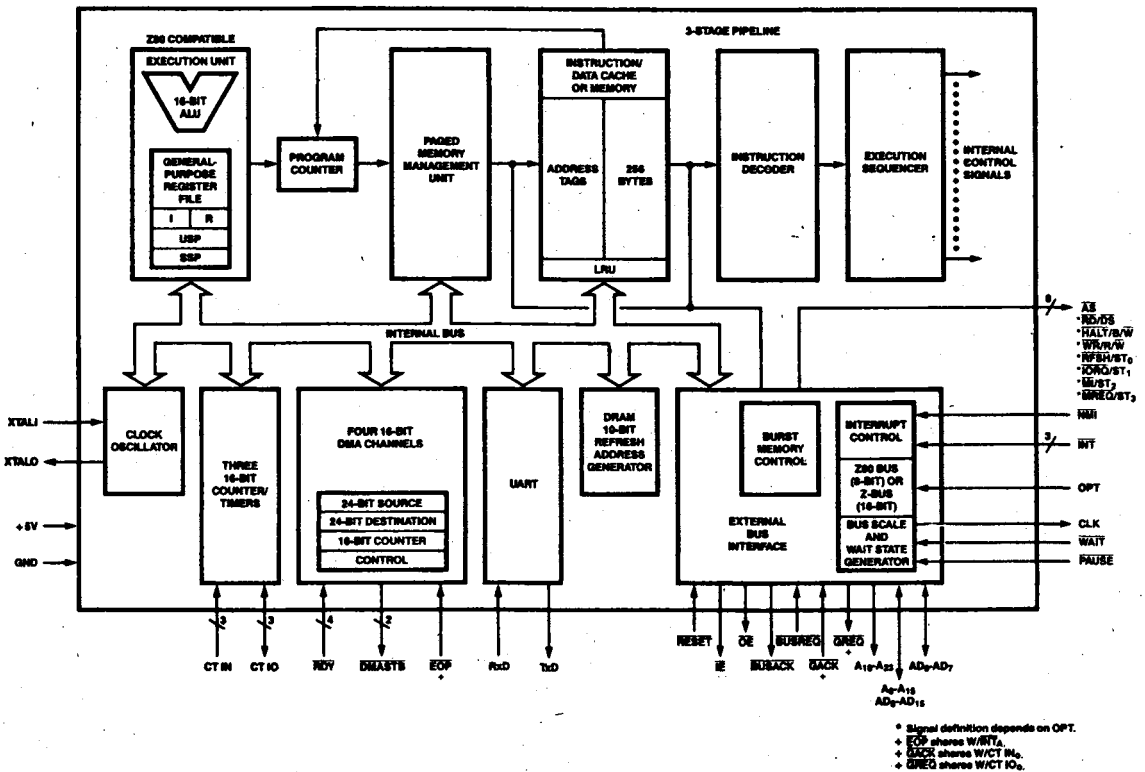
Figure 1-1. Block Diagram
