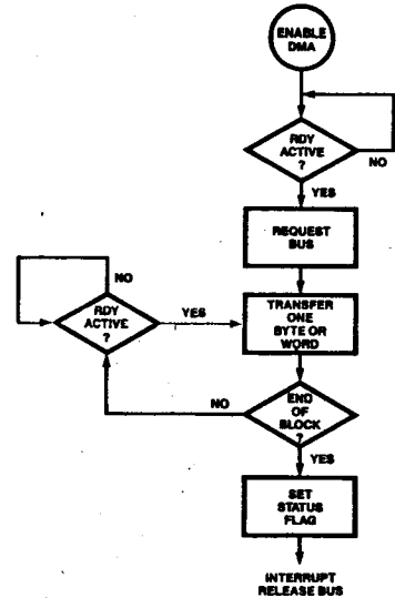
Figure 9-8c. Continuous Mode
