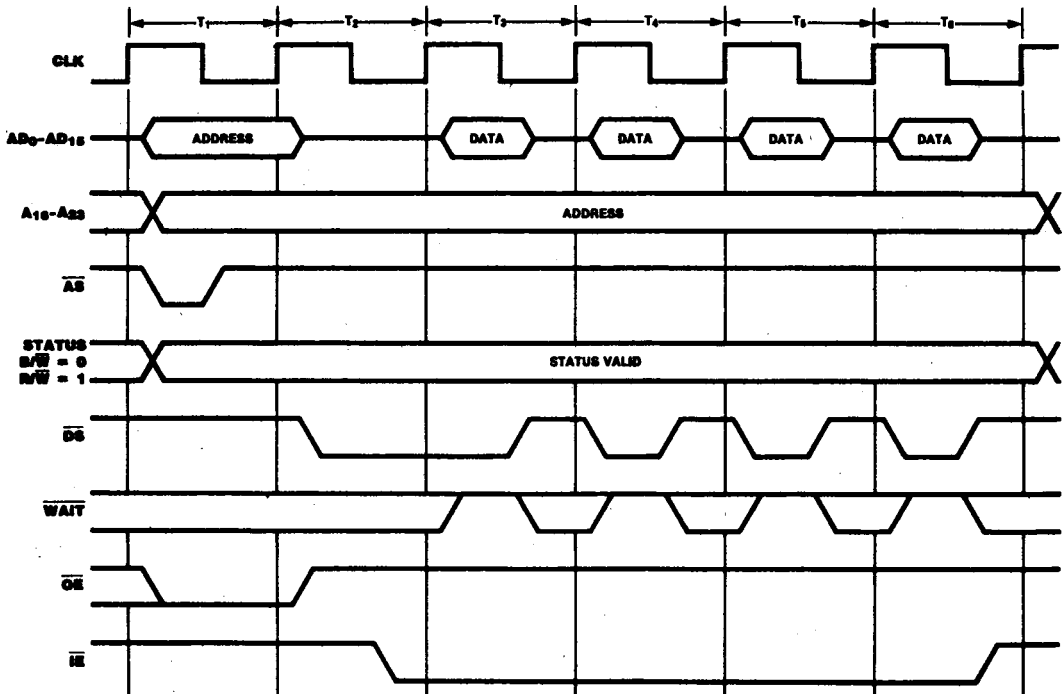
Figure 13-7. Burst Memory Read Timing
