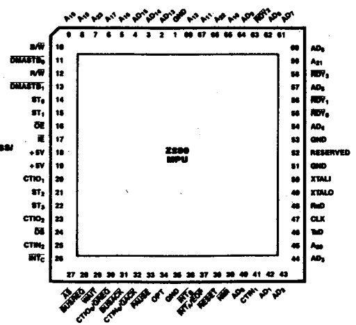
Figure 13-1b. Pin Assignments
