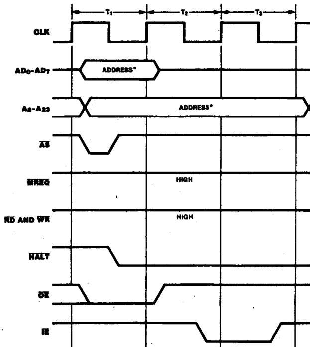
Figure 12-8. Halt Timing
