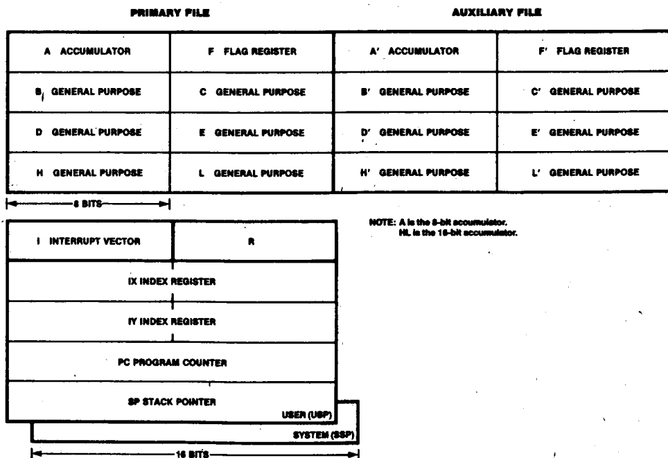
Figure 2-1. Register File Organization
