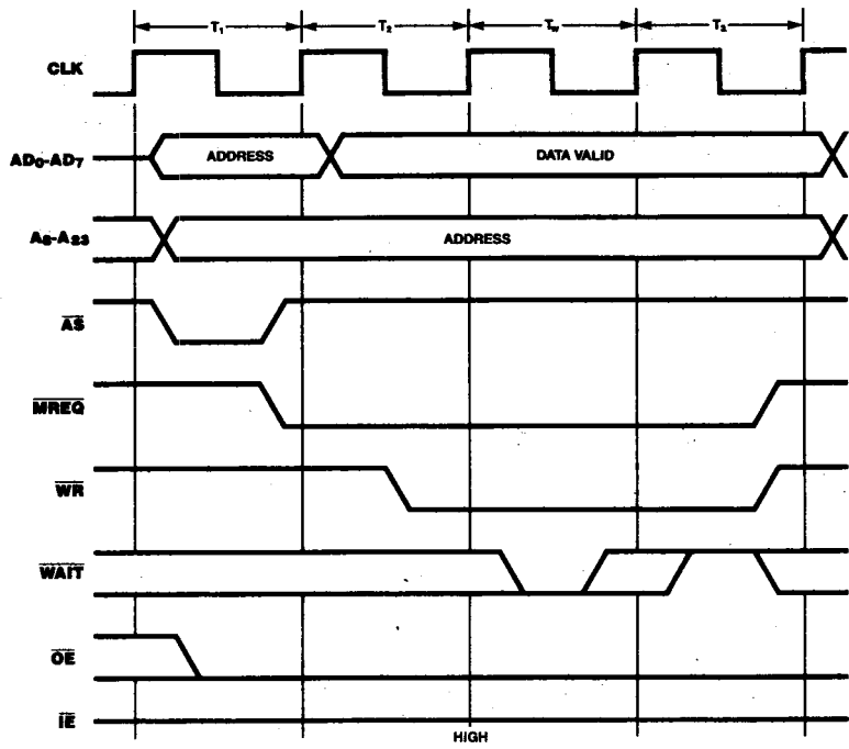
Figure 12-5. Memory Write Timing with One External Wait State
