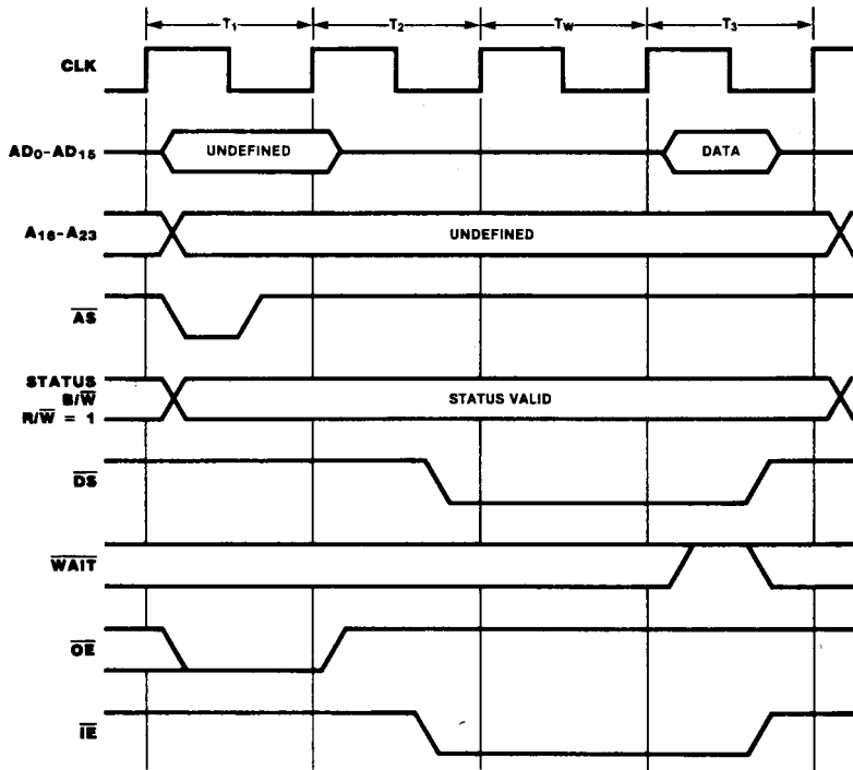
Figure 13-15. EPU to CPU Timing
