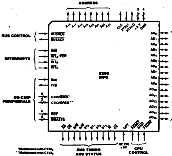
Figure 13-1a. Pin Functions
