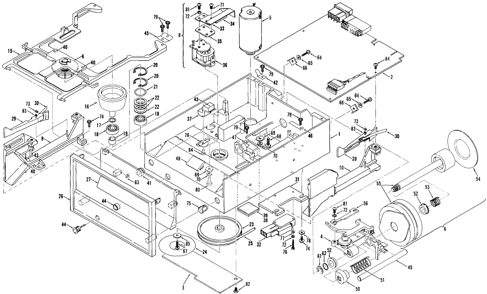
Figure D-1. Model FDD100-5B Disk Drive — Overall View
