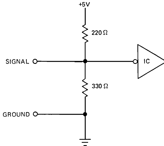
Figure 2-6. Termination Configuration
