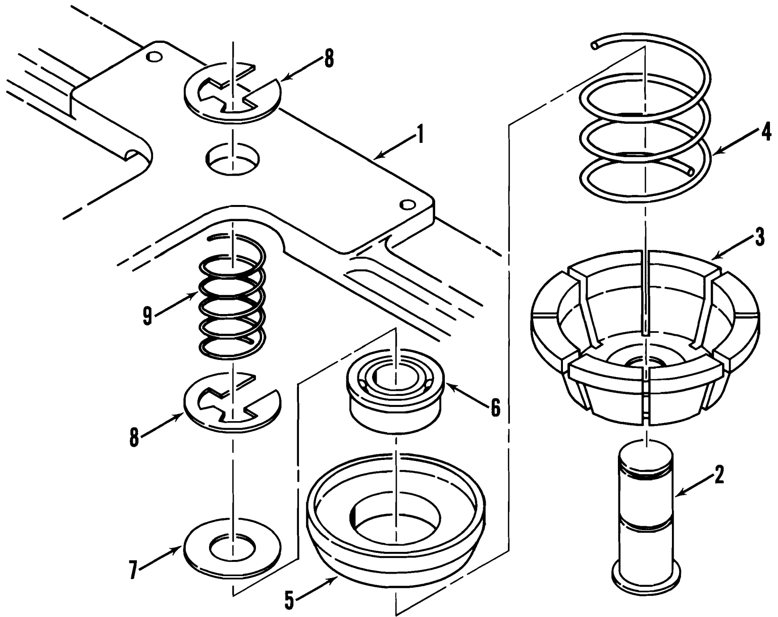
Figure D-2. Model FDD100-5 – Clutch Assembly
