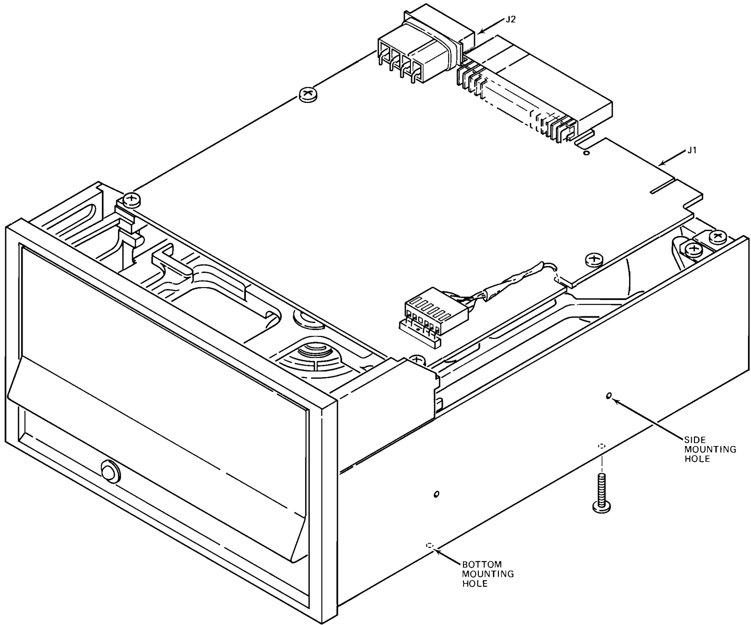
Figure 2-1. Model FDD100-5 Disk Drive, Isometric View
