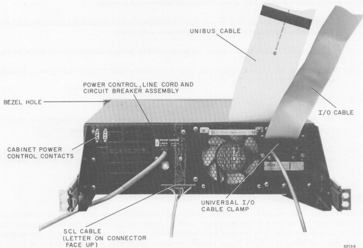
Figure 3-7 Rear of Computer With Cable Strain Reliefs
