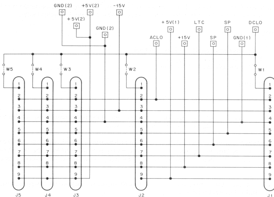
Figure 19-13 Power Distribtuion Board Circuit Schematic
