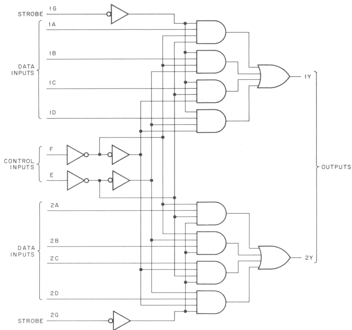
LOGIC DIAGRAM
