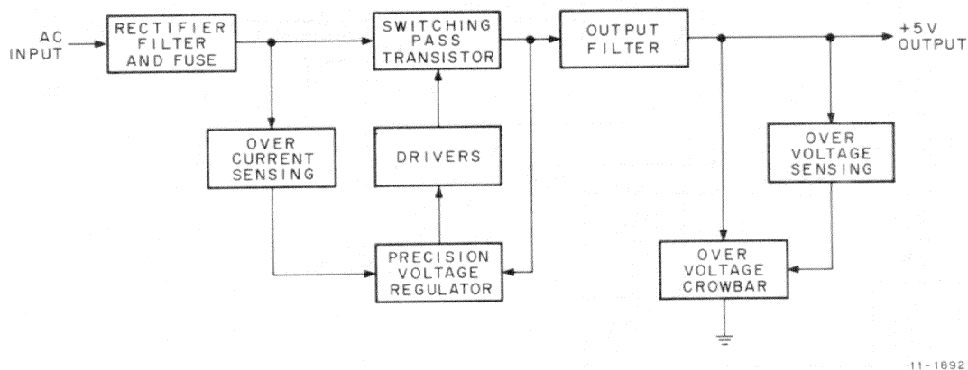
Figure 19-20 +5 V Regulator (PS2) Functional Block Diagram
