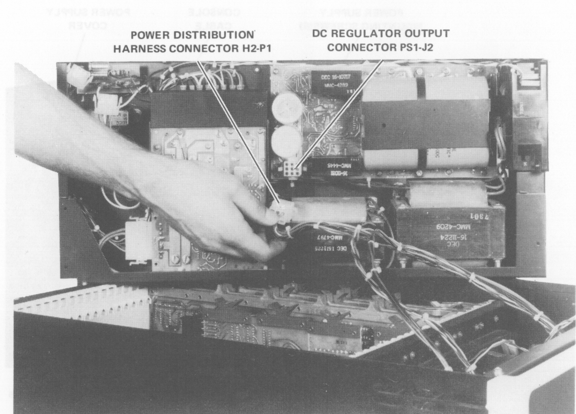
Figure 19-29 Disconnecting DC Regulator Output Connector
