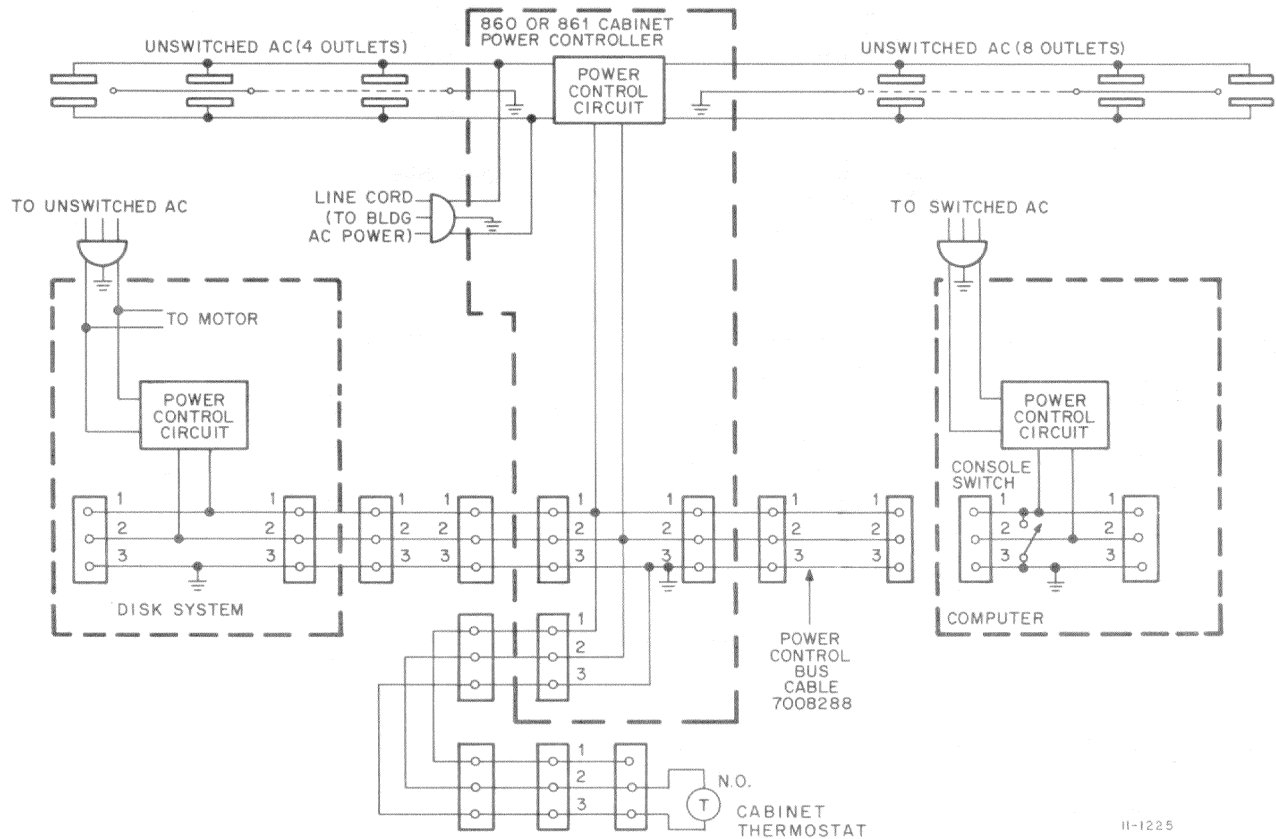
Figure 18-4 Typical Cabinet Power Control System Wiring Diagram
