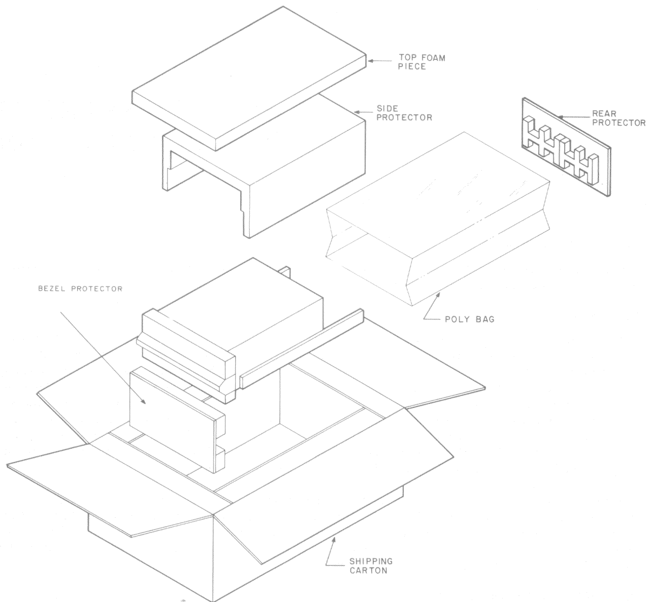
Figure 18-1 Computer Packaging
