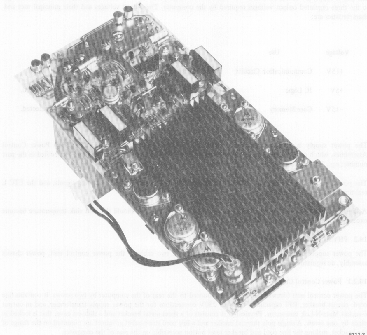
Figure 14-1 Power Chassis Assembly (with DC Regulator Module)
