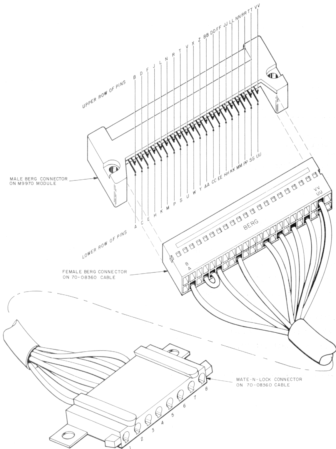
Figure 18-2 SCL Cable 70-08360
