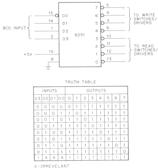
Figure 12-9 Type 8251 Decoder, Pin Designation and Truth Table
