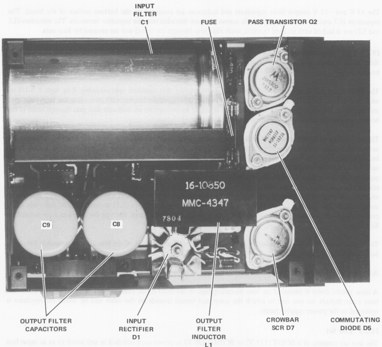
Figure 19-5 +5 V Regulator, Side View
