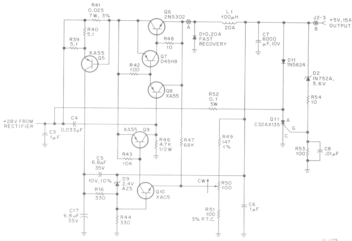
Figure 15-8 +5V Regulator Circuit
