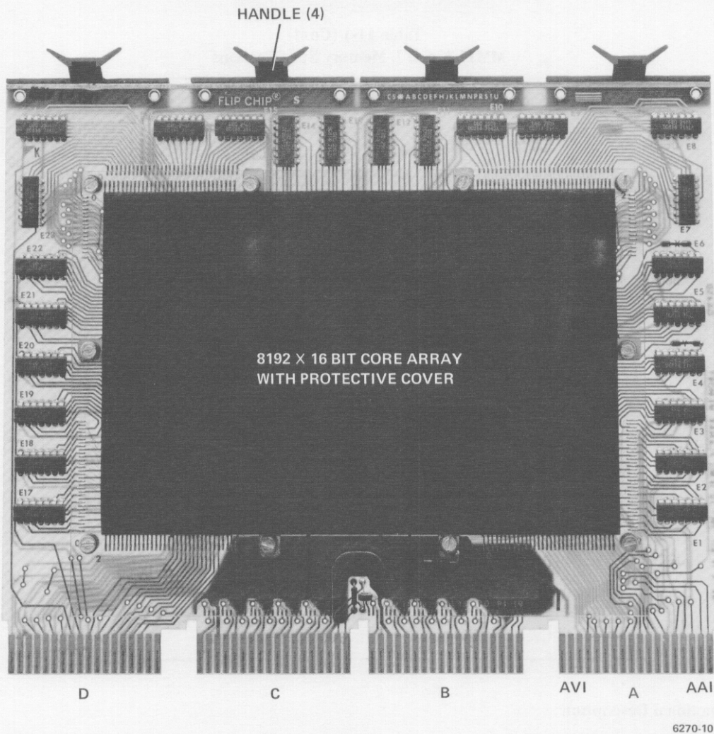
Figure 11-3 Component Side of 8K H214 Stack Module
