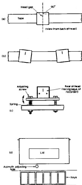
Fig. A7. Tape-head azimuth. The narrow slit in the tape-head (a) is normally at 90^\circ to the edge of the tape. This is the correct azimuth angle, but a surprising number of recorders have this maladjusted. Any deviation from this angle (b) causes muffled sound and poor loading. The angle can be altered by turning an adjusting screw (c) which is on the head mounting. This is often reached through a hole in the casing of the recorder (d). (Courtesy of Keith Dickson Publishing.)
