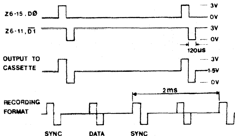
Fig 1.12 Cassette Write Signals
