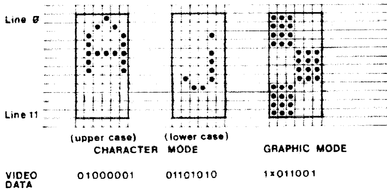
Fig 1.10 Character/Graphic Display Format
