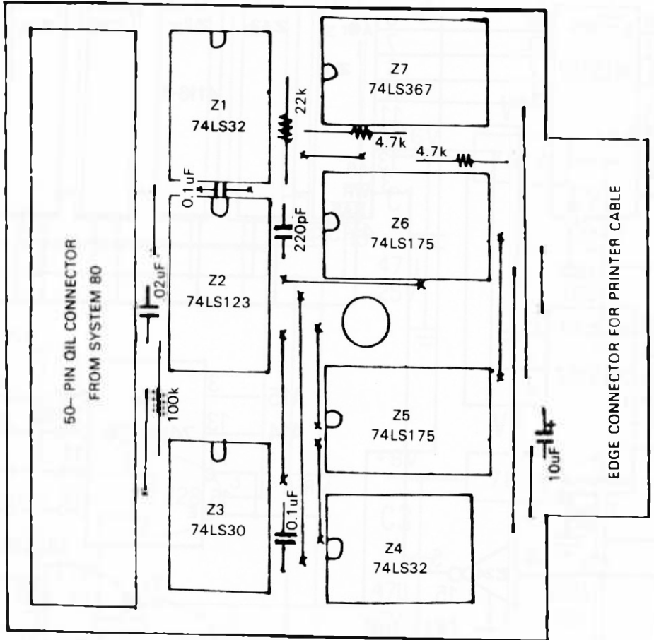
PARALLEL PRINTER INTERFACE X-4013 COMPONENT LAYOUT ON PCB
