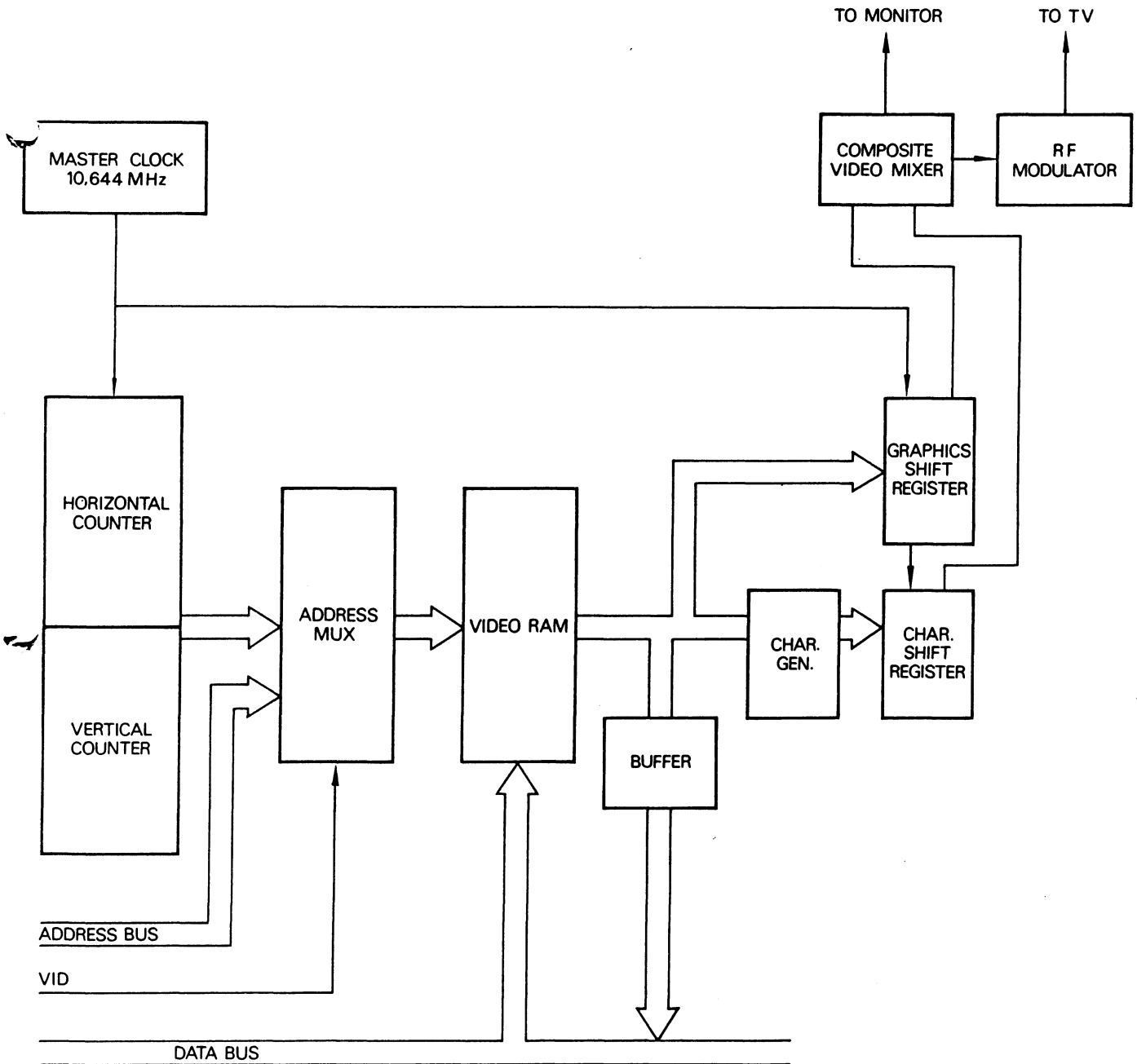
Fig. 4. VIDEO INTERFACE BLOCK DIAGRAM
